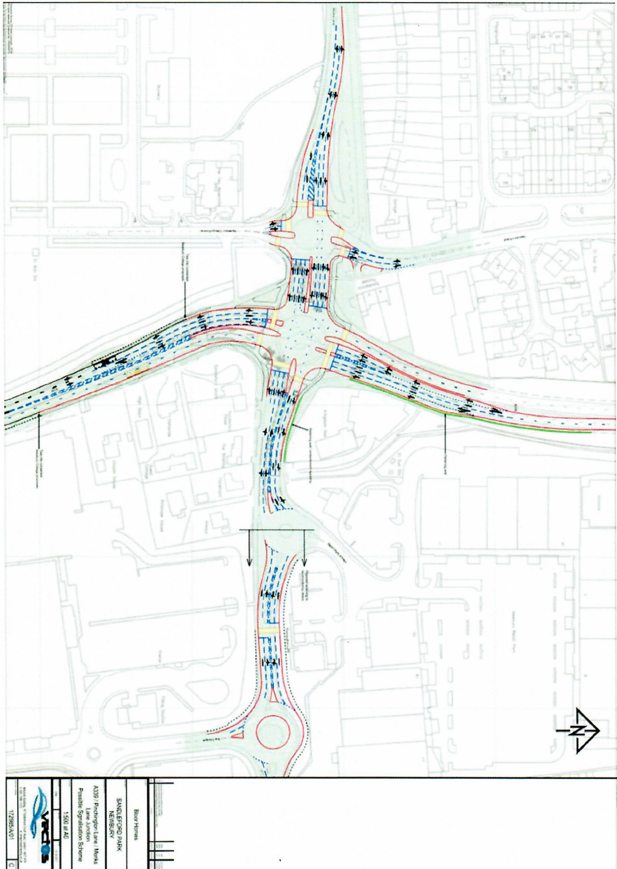
Figure C-2 - A339 / Pinchington Lane / Monks lane layout v2
